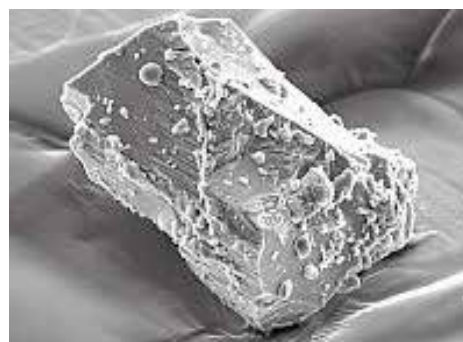
初期分析を行ったはやぶさ回収粒子 A lithic particle returned by Hayabusa spacecraft, which is analyzed by us.
